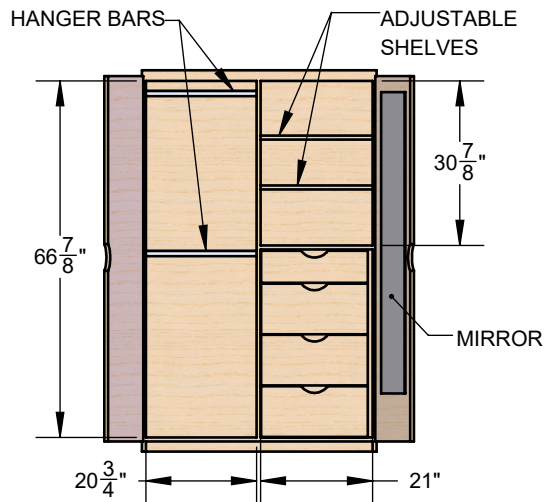
WARDROBE DETAIL
